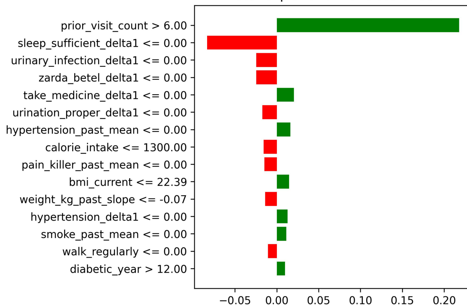
False negative LIME
