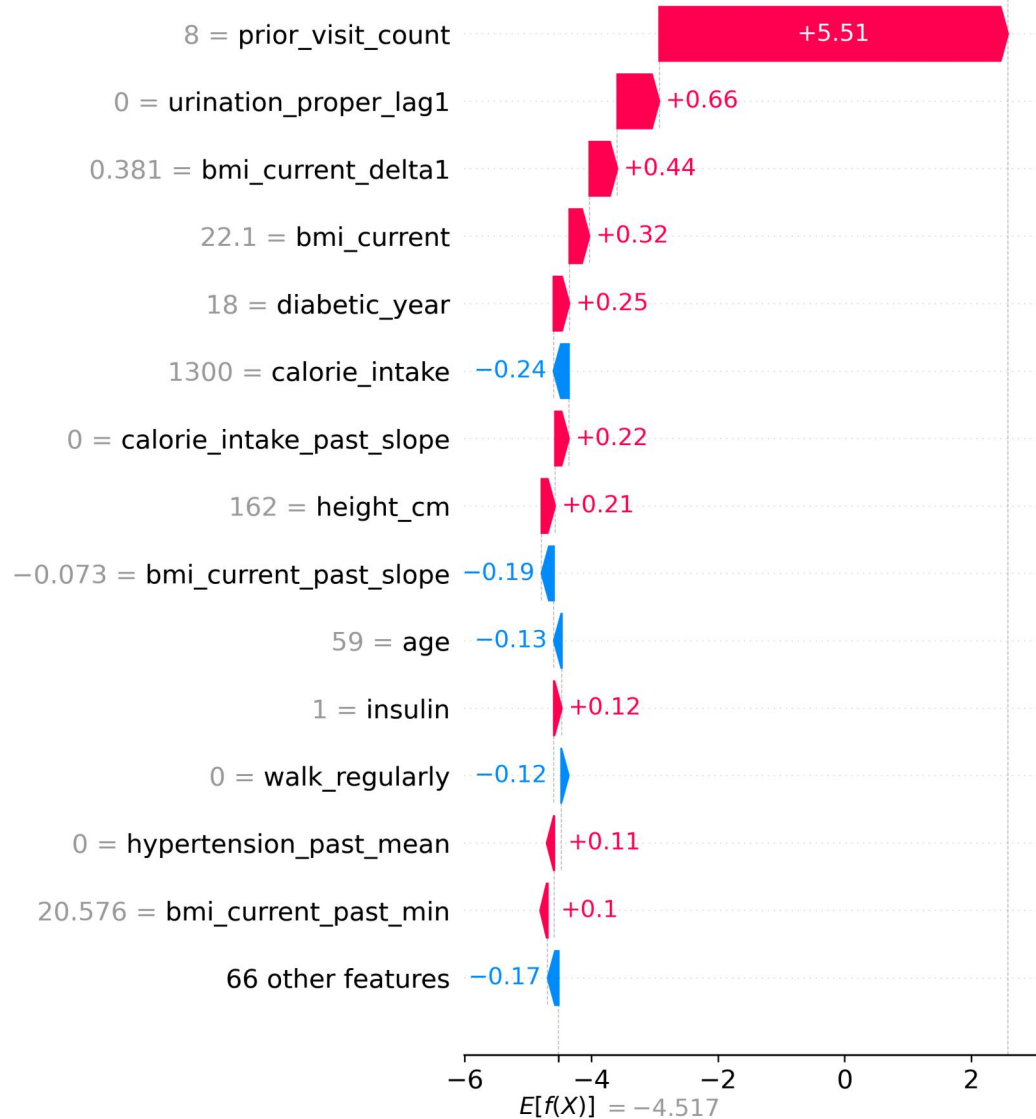
False negative SHAP
